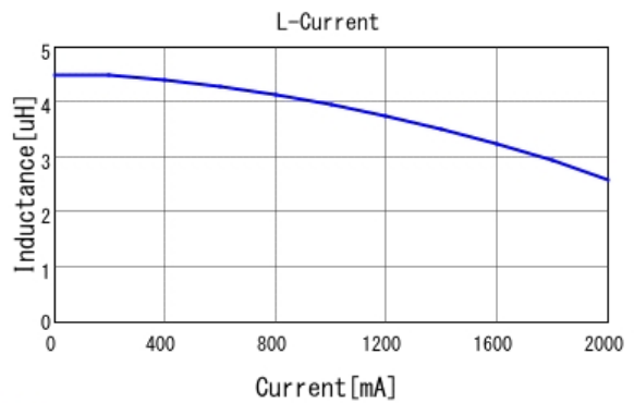
■ 1269AS-H-4R7M L-Current 20degC
